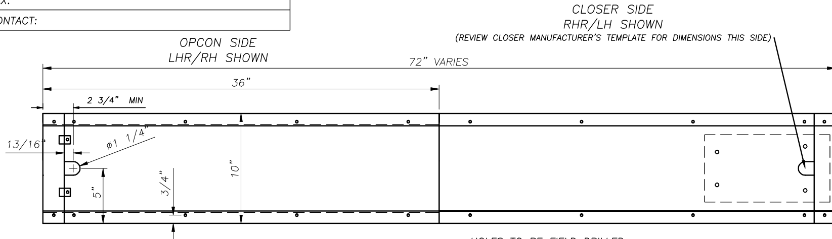
TYPICAL CENTER HUNG PREP FOR ONE OPCON (LHR/RH) AND ONE MANUAL CLOSER (OR OPPOSITE) ON 72" PAIR OF DOORS TOP VIEW (REMOVABLE "B" SECTION, STRAIGHT EDGE)
