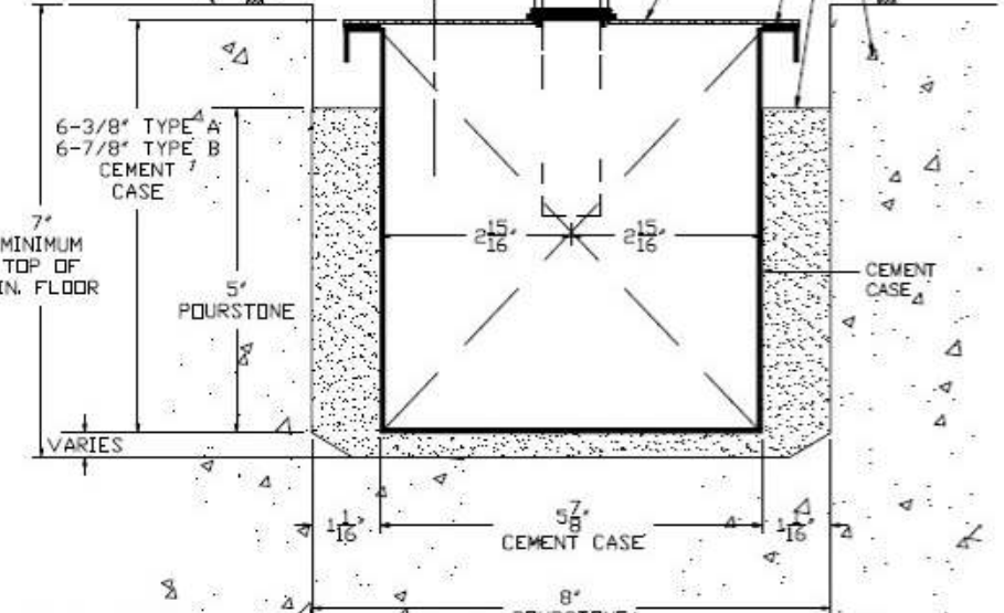
1.0 END SECTION VIEW
