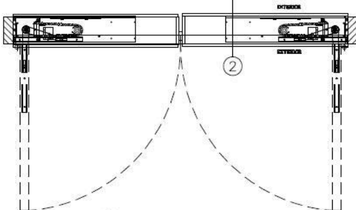
PLAN ① SCALE = 1:20
