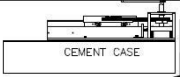
CEMENT CASES SHOWN BELOW SLEDS FOR CLARITY FRONT ELEV. ③ SCALE = 1:20
