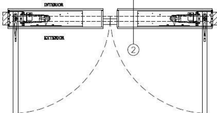
PLAN ① SCALE = 1:20
