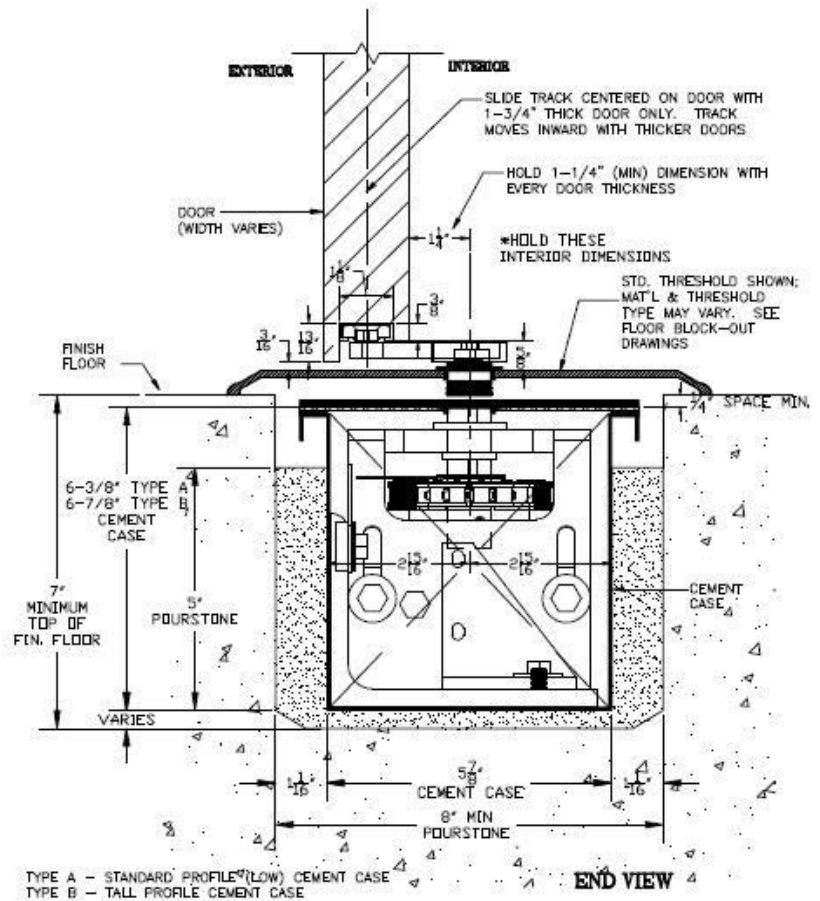
SECTION ② OFFSET PIVOT
