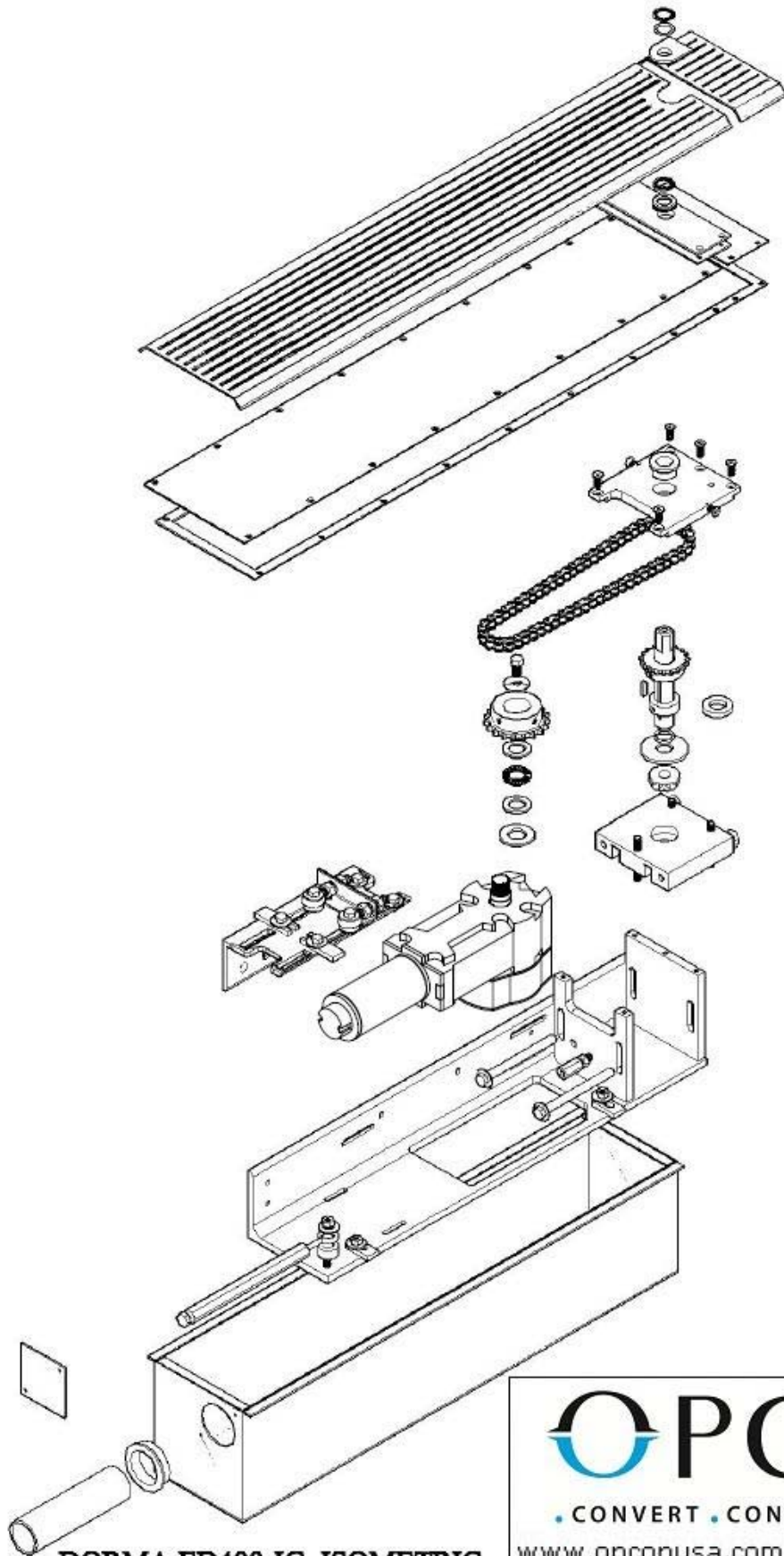
DORMA ED400-IG ISOMETRIC
