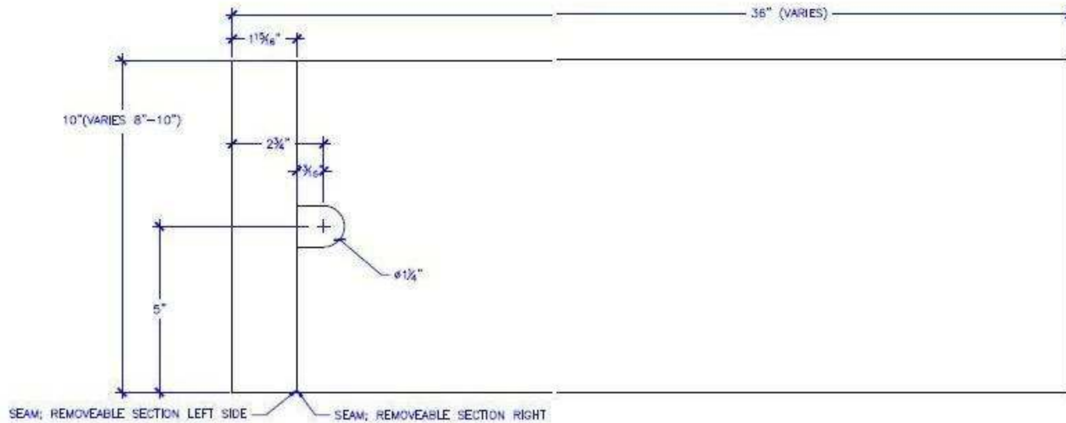
PLAN VIEW
